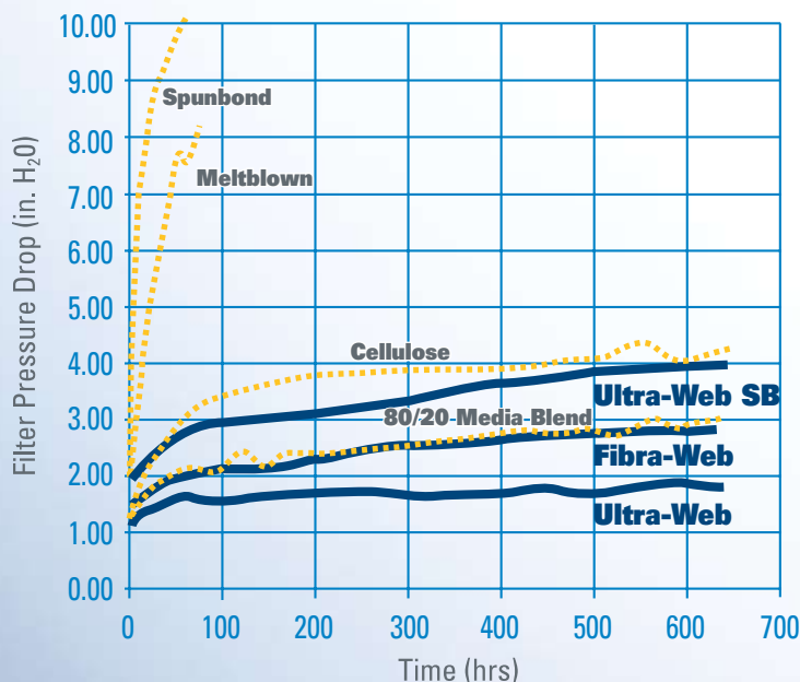
LOWER PRESSURE DROP = LONGER FILTER LIFE
